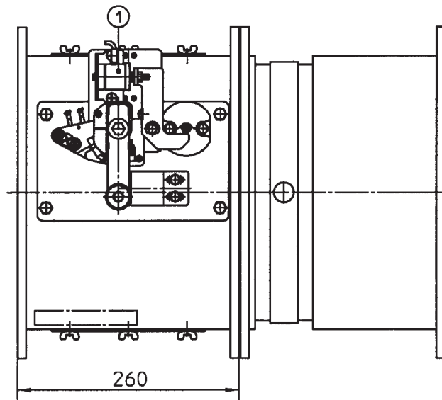
① Magnet
