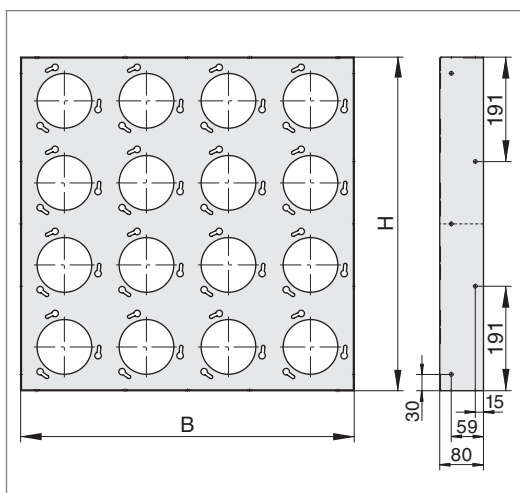
Detail drawing 1: Mounting plate for activated carbon filter cartridges
